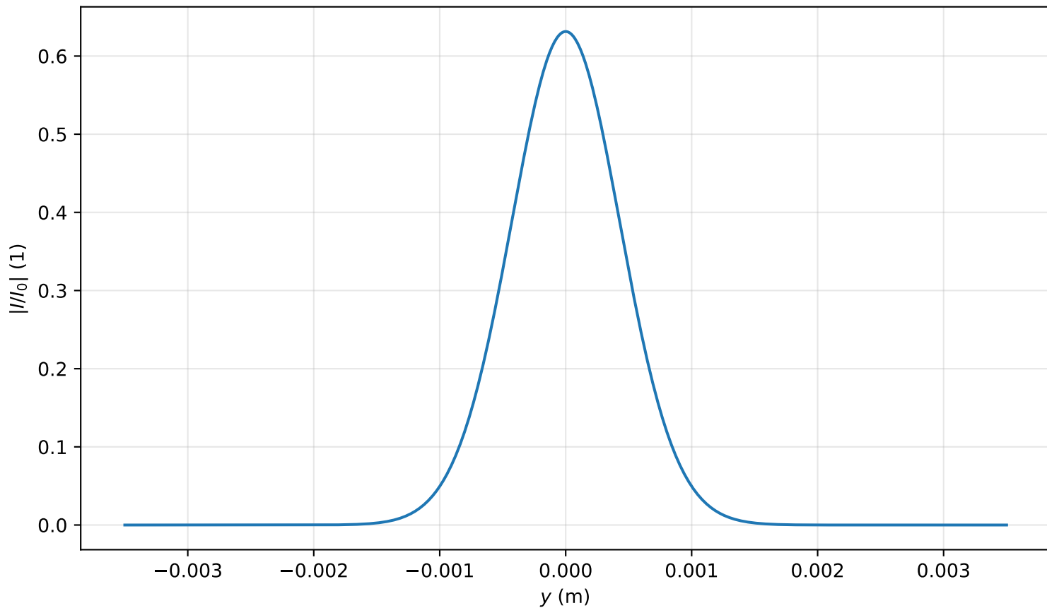
Intensity profile I(x=0, y, z=1.672)/I_0 , P_{in}=0.1P_{cr} , artificial time
